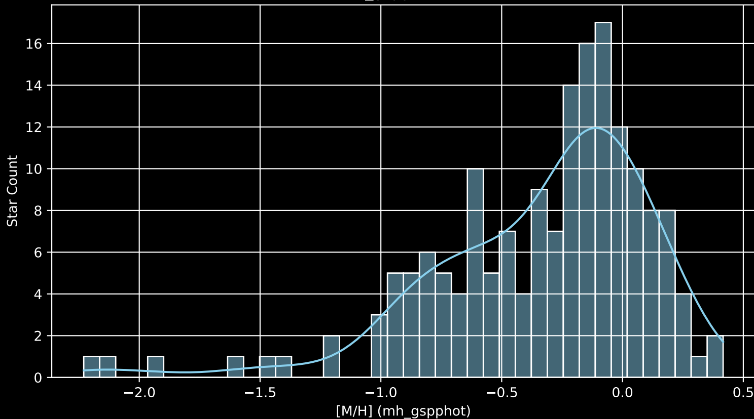
APOGEE DR17 Field: [351+24-O [M/H] (mh_gspphot) (n= 170)
