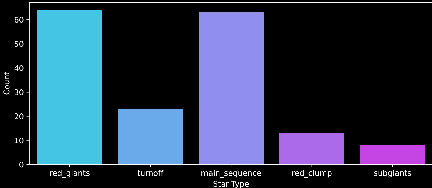
APOGEE DR17 Field: [351+24-O] Count plot of Star Type
