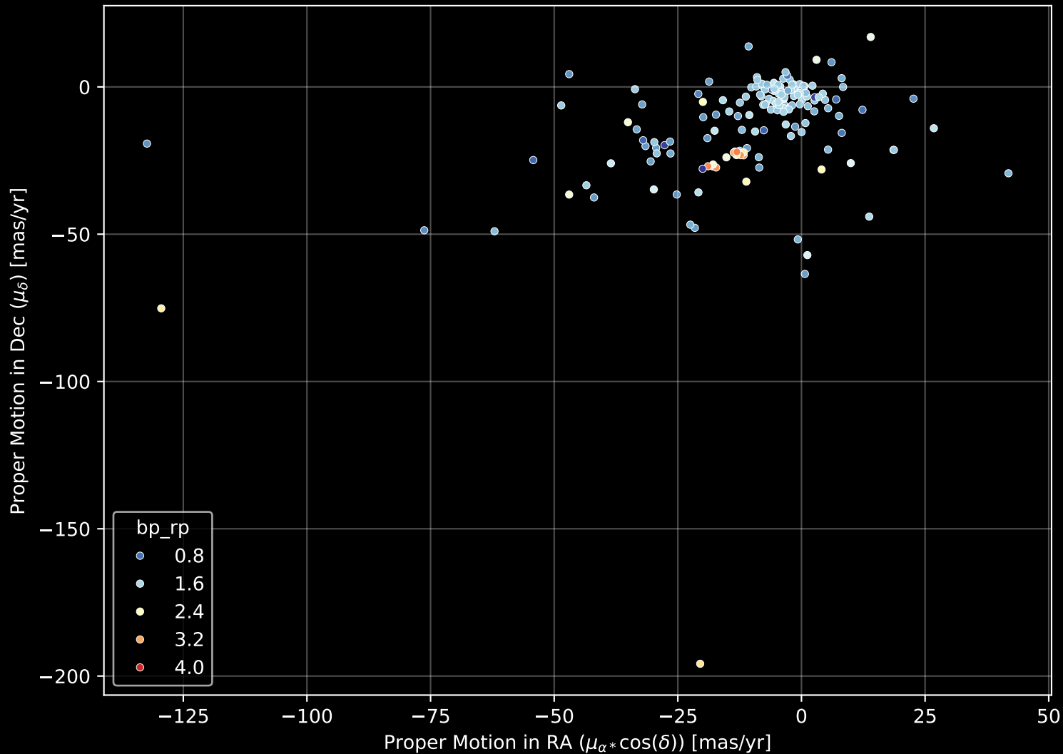
APOGEE DR17 Field: [351+24-O] Proper Motion Diagram (n= 171)
