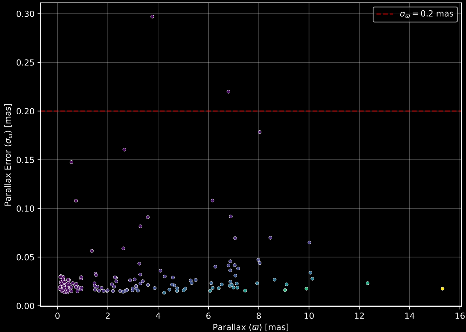
APOGEE DR17 Field: [351+24-O] Parallax Quality (n= 171)
