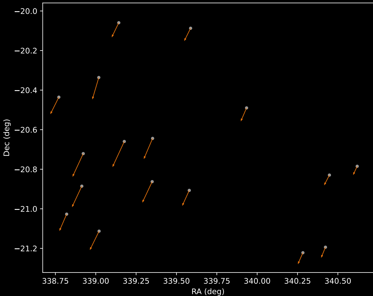
APOGEE DR17 Cluster 2 Proper Motion Vectors (n=17)
