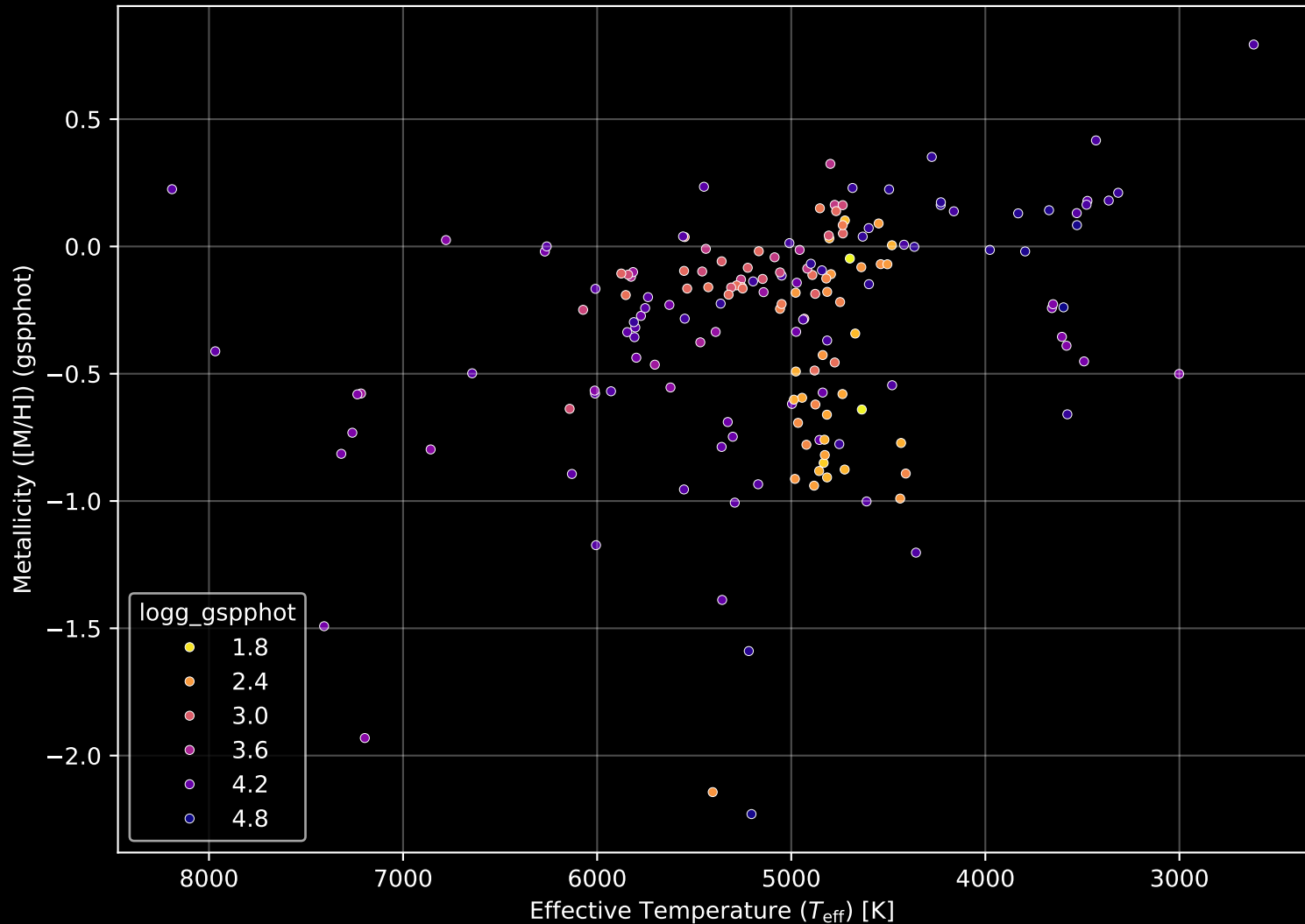
APOGEE DR17 Field: [351+24-O] Stellar Population Parameters (n= 171)
