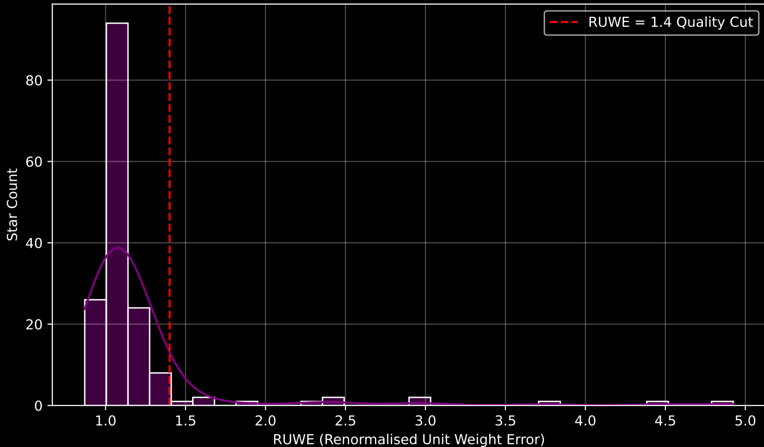
GAPOGEE DR17 Field [351+24-O] RUWE Distribution (n= 164)
