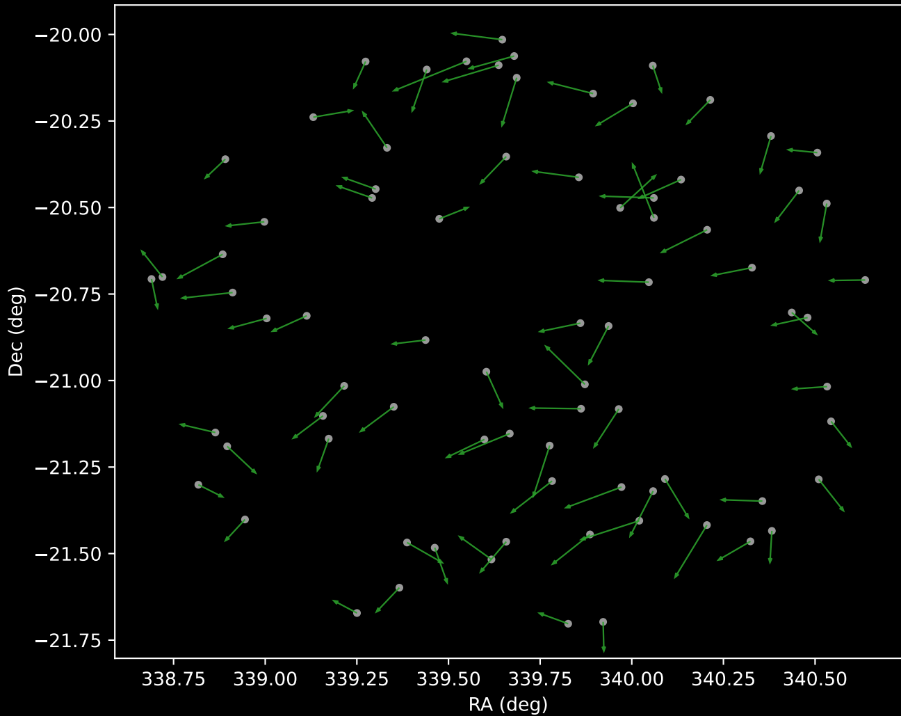
APOGEE DR17 Cluster 4 Proper Motion Vectors (n=79)
