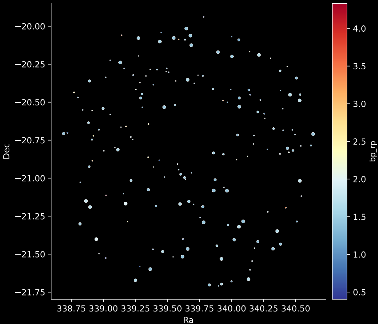
APOGEE DR17 Field: [351+24-O] Stars: 171
